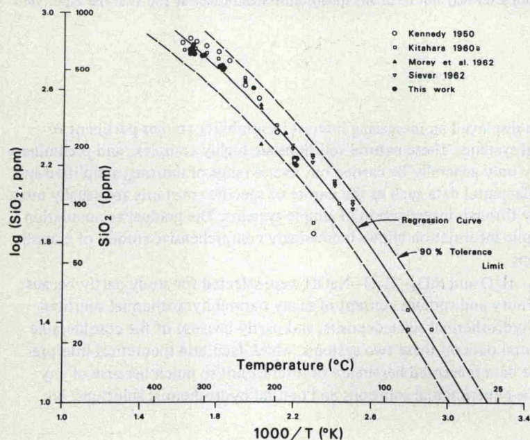
Fig. 1. Least squares quadratic fit to all published solubility data for the three-phase subcritical region of the quartz-water system up to 325°C.
